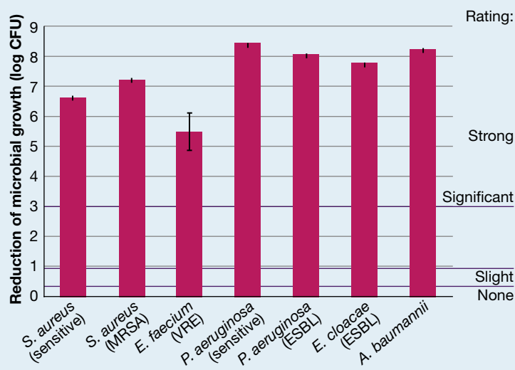
Fig 3. Testing of the antibacterial activity of the dialkylcarbamoyl chloride-coated dressing according to JIS L 1902 showed a strong antibacterial activity against the WHO-prioritised bacteria strains. CFU—colony forming units; S. aureus — Staphylococcus aureus ; P. aeruginosa — Pseudomonas aeruginosa ; E. cloacae — Enterococcus cloacae ; A. baumannii — Acinetobacter baumannii ; ESBL—extended-spectrum beta-lactamase; MRSA—meticillin-resistant Staphylococcus aureus ; VRE—vancomycin-resistant Enterococcus
